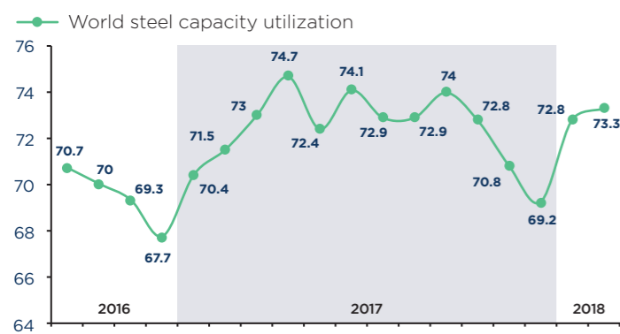
Graph 11: Capacity Utilization (%)
